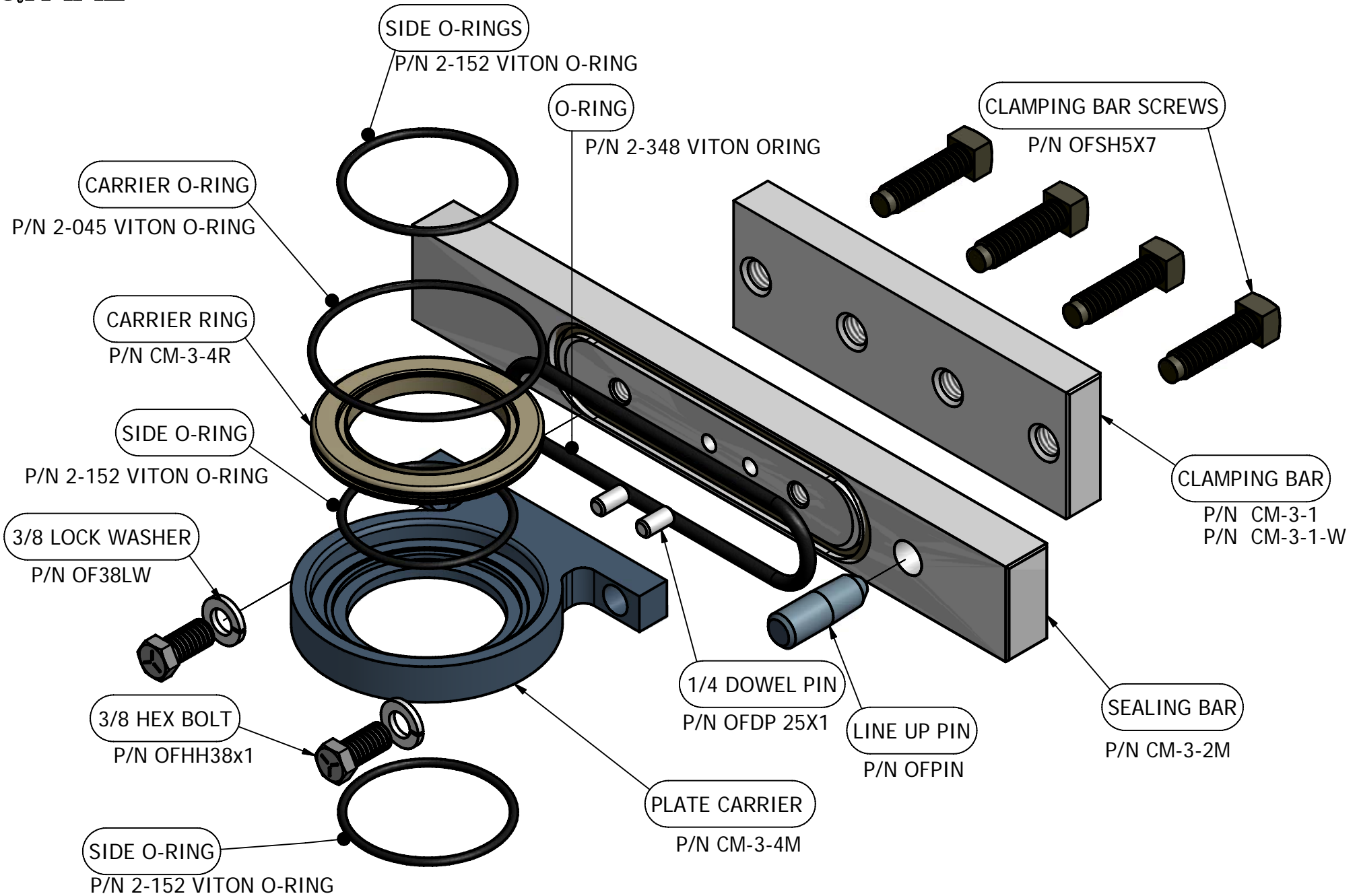
3 INCH PLATE CARRIER ASSEMBLY NEW STYLE AGA-2000
